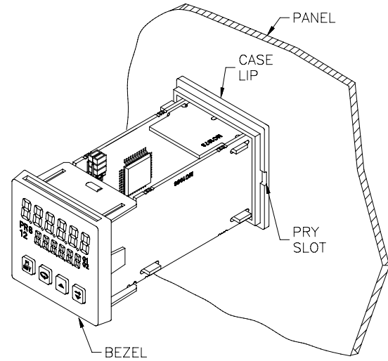
Figure 4, Unit Assembly
