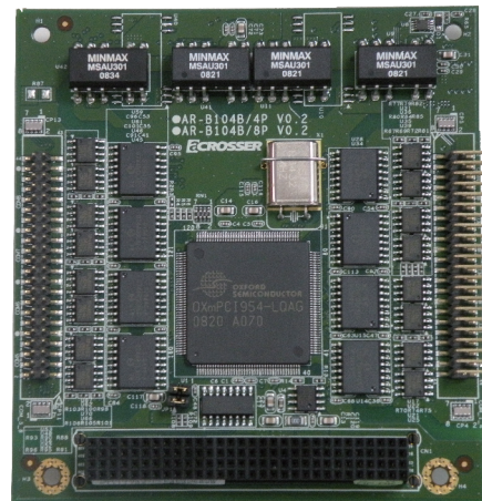
AR-B104B/8P AR-B104B/4P
