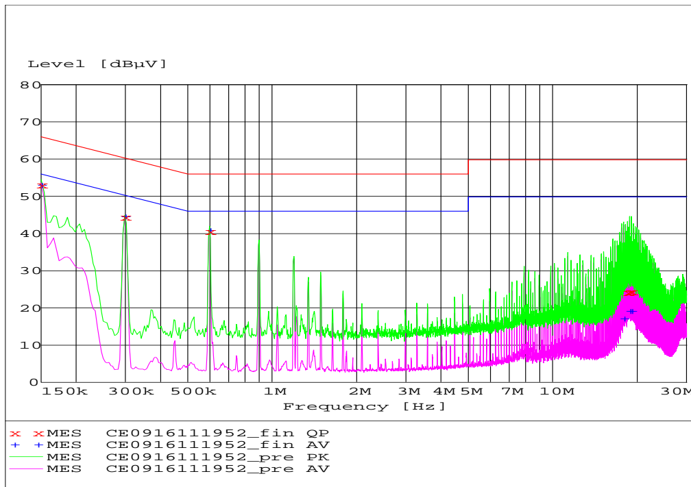
Figure 25. EMC Considerations.
