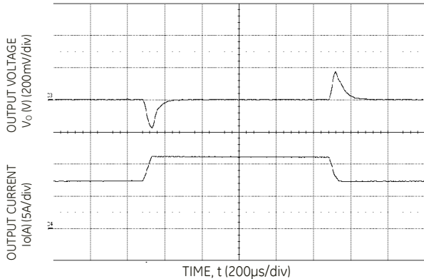
Figure 3. Transient Response to 0.1A/μs Dynamic Load Change from 50% to 75% to 50% of full load, Vin=48V, Co>100μF.
