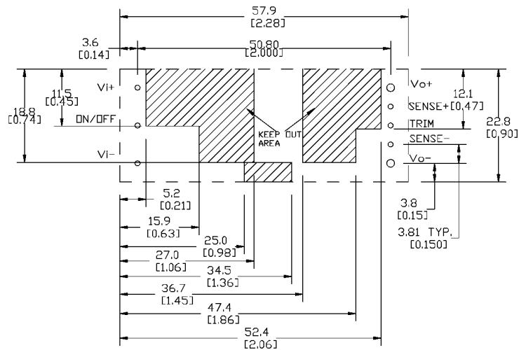
TH Recommended Pad Layout (Component Side View)
