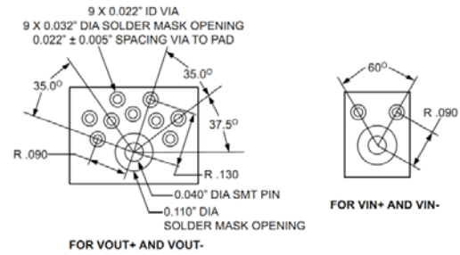
SMT Recommended Pad Layout (Component Side View)
