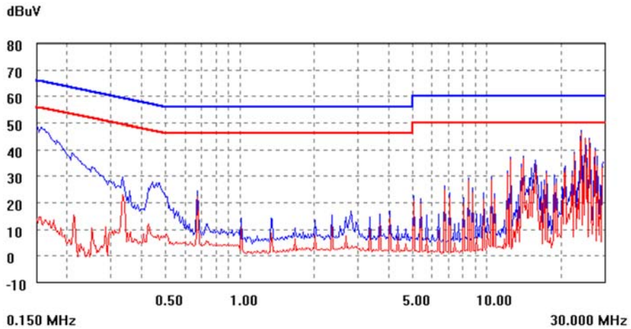
Figure 25. EMC Considerations
