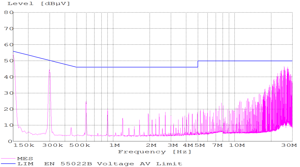
Figure 25. EMC Considerations
